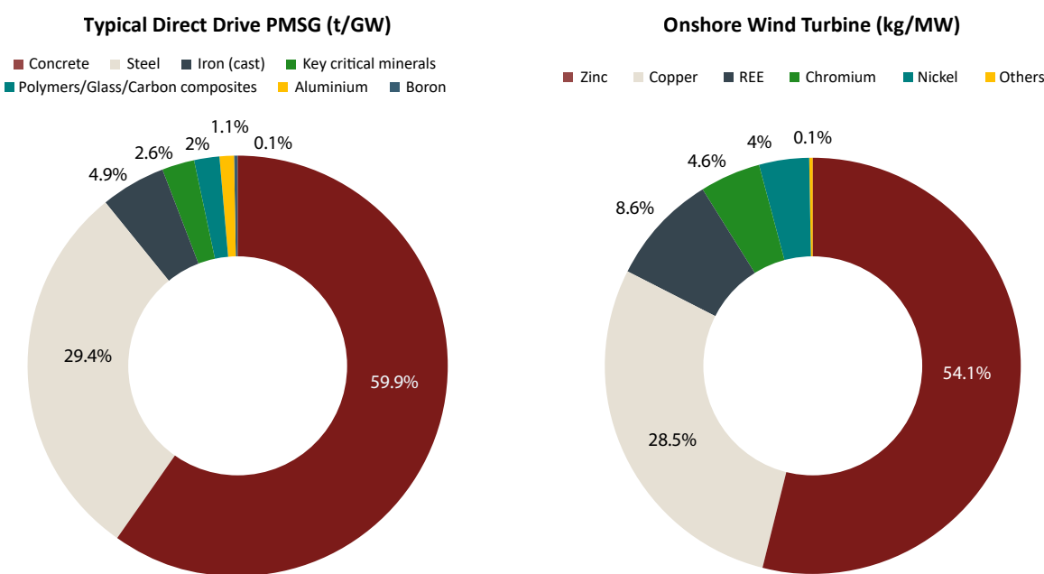
Figure 38: Material breakdown of onshore wind turbines
